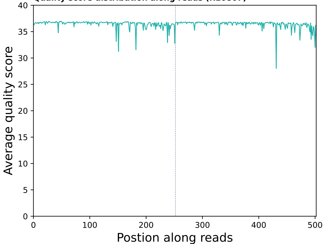
Quality score distribution along reads (R10807)
